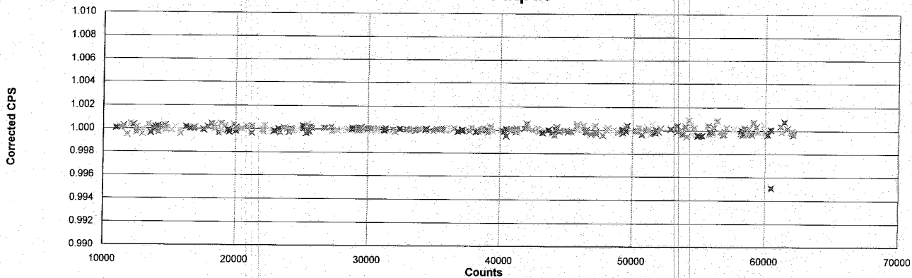
Linearized Output
