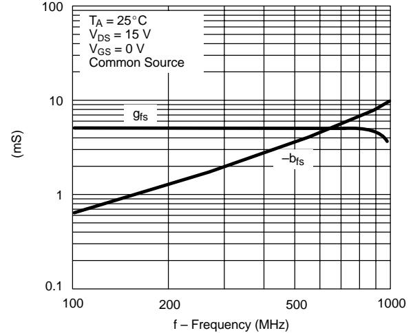
Forward Admittance
