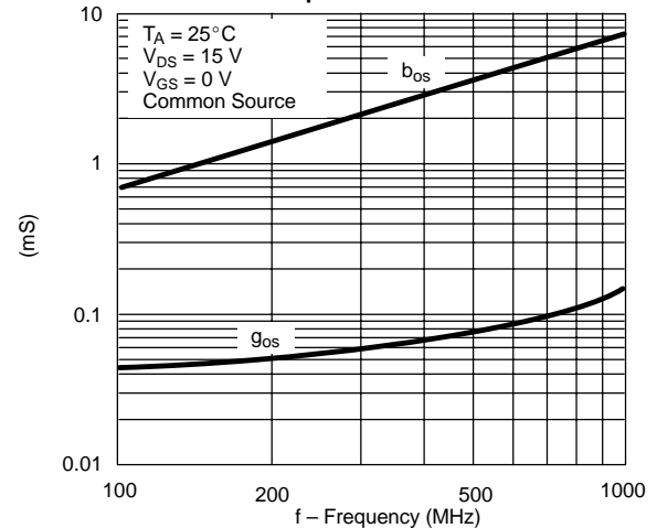
Output Admittance
