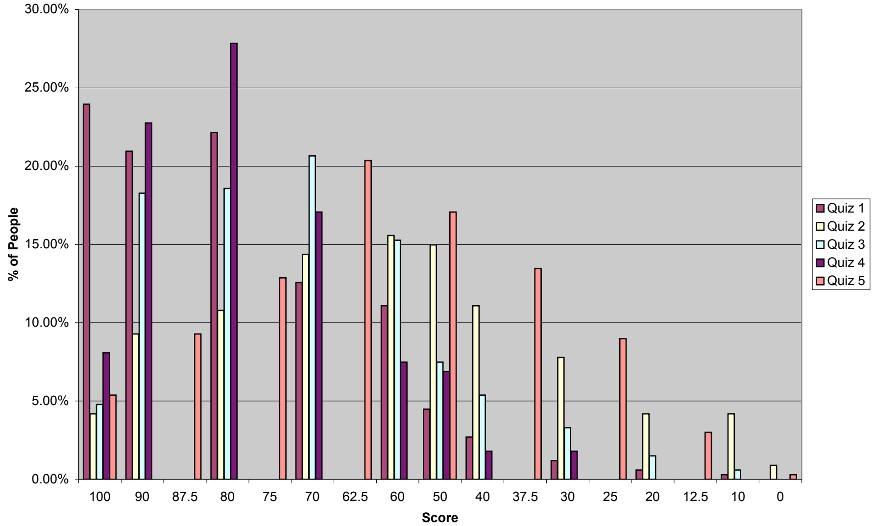
Histogram
