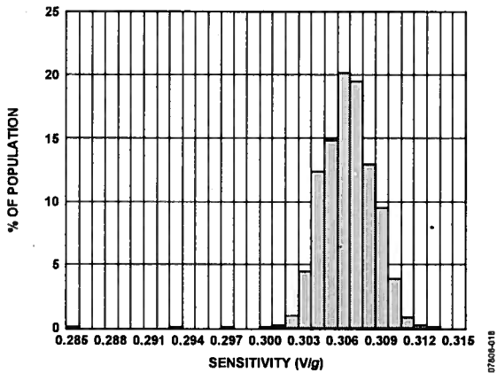
Figure 16. Y-Axis Sensitivity at 25°C, V_S = 3V
