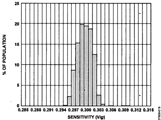
Figure 17. Z-Axis Sensitivity at 25°C, V_S = 3V
