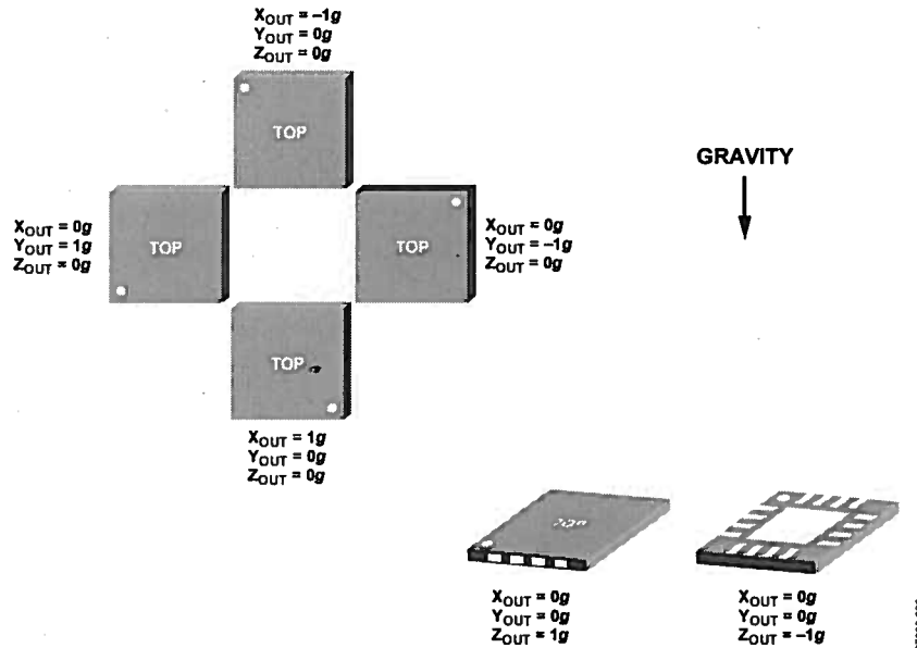
Figure 24. Output Response vs. Orientation to Gravity
