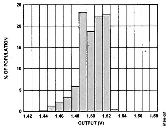
Figure 5. Z-Axis Zero g Bias at 25°C, V_S = 3 V
