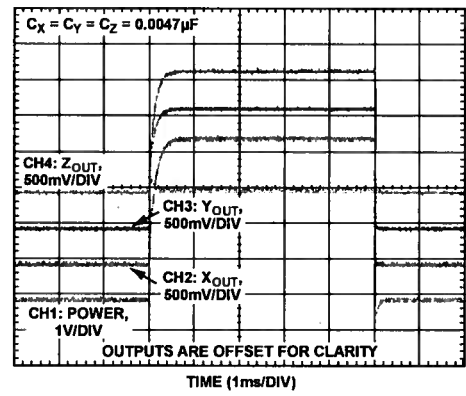
Figure 22. Typical Turn-On Time, V_S = 3\text{ V}
