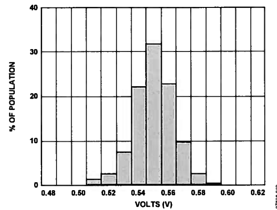
Figure 8. Z-Axis Self-Test Response at 25°C, V_S = 3 V
