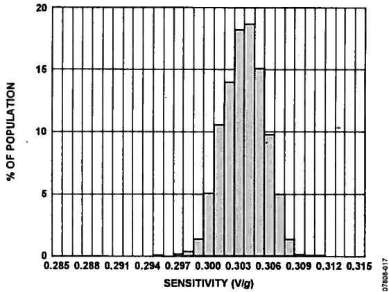
Figure 15. X-Axis Sensitivity at 25°C, V_S = 3V
