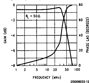
Frequency Response
