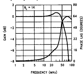
Frequency Response
