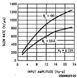
Slew Rate
