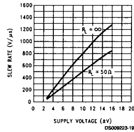
Slew Rate
