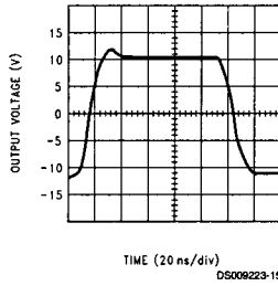
Large Signal Response R_L = 1\text{ k}\Omega
