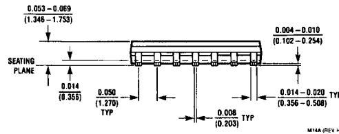
14-Pin Small Outline Package (M) Order Number LM6321M NS Package Number M14A
