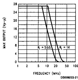
Power Bandwidth
