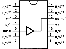
Plastic SO
