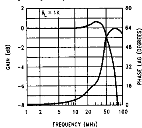
Frequency Response
