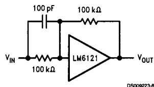
FIGURE 1. LM6121 with Overvoltage Protection
