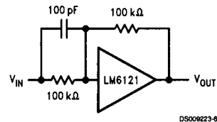
FIGURE 1. LM6121 with Overvoltage Protection
