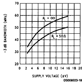
-3 dB Bandwidth
