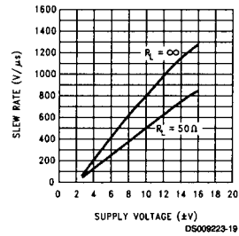
Slew Rate
