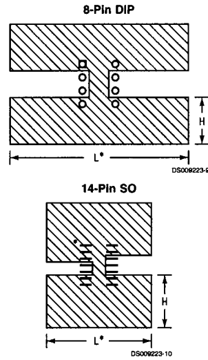
FIGURE 3. Copper Heatsink Patterns TABLE 2.
