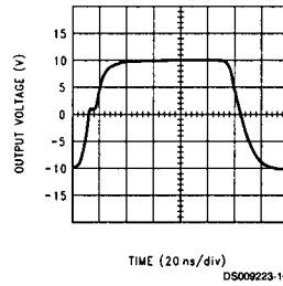
Large Signal Response R_L = 50\Omega
