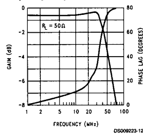
Frequency Response
