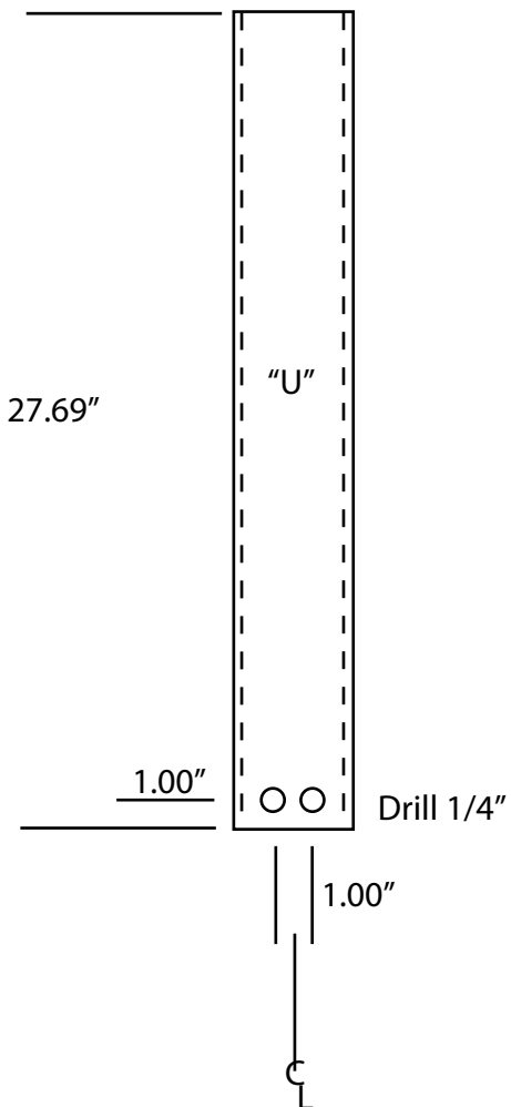
2-0" by 4-0" by 0-1/4" aluminum "U"
