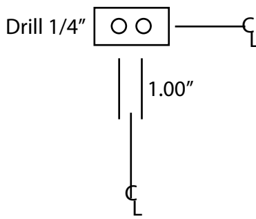
2-0" by 4-0" by 0-1/4" aluminum plate
