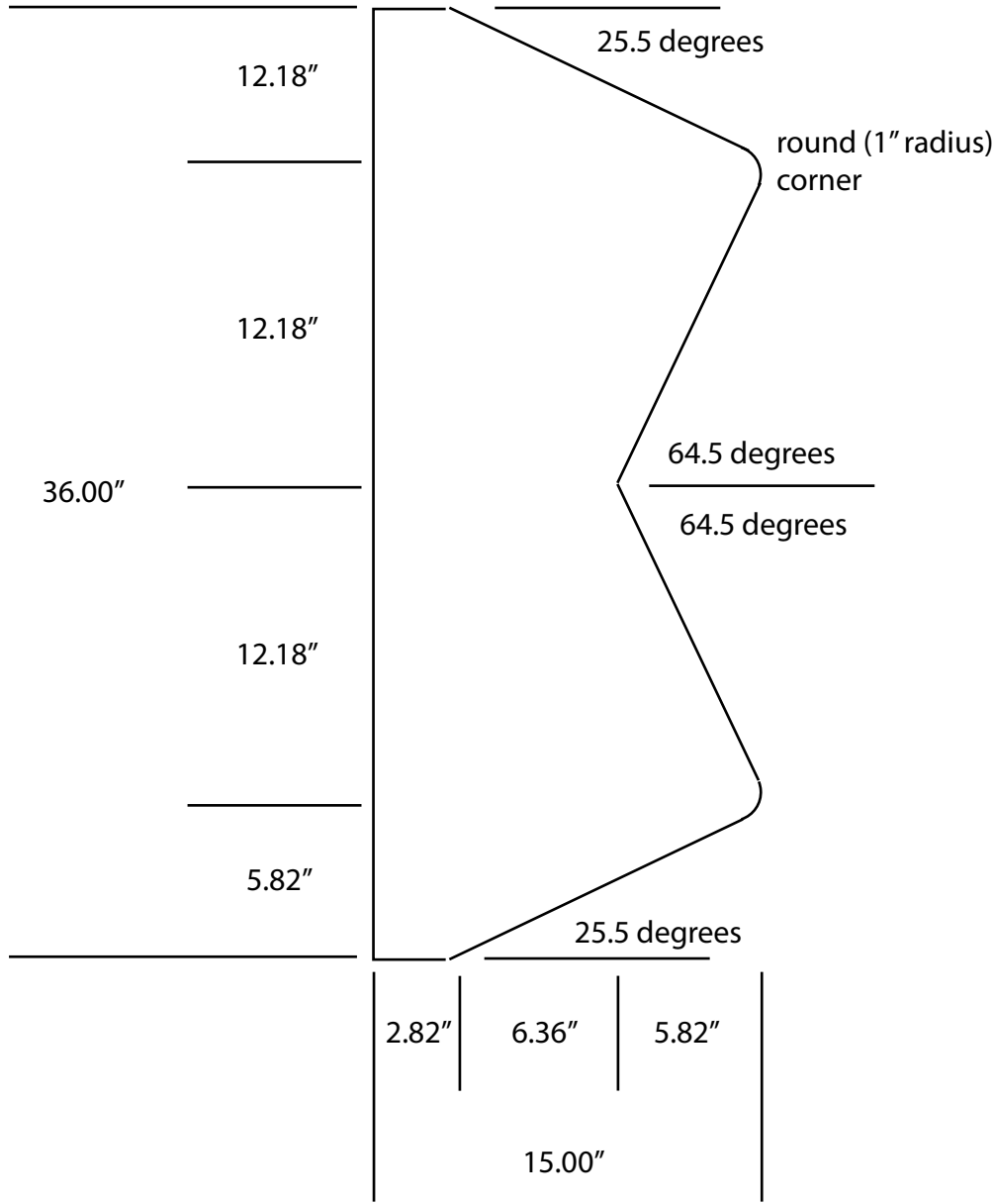
Material: 3/16" aluminum
