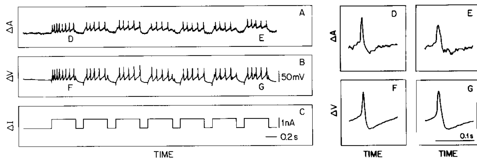
FIGURE 2 Simultaneous optical and intracellular recordings of repetitive action potentials in a cultured LUQ neuron. The cell was bathed in deoxygenated ASW. Action potentials were induced by injecting intracellular pulses of current. (A) Optical record, \Delta A , of the first 7 s of activity. Note that the decrease in the number of action potentials during the first current pulse is caused by spike adaptation. (B) Intracellular record, \Delta V , of the first 7 s of activity. (C) Record of the intracellular current, \Delta I(t) . Pulses were 2 nA in amplitude, 600 ms in duration and repeated every 800 ms. (D-G) Comparison of the records for individual action potentials occurring at the beginning and end of the measurements. This illustrates the integrity of both the optical and the electrical signal after sustained firing. The optical record for the seventh action potential (D) is to be compared with the concomitant intracellular record (F). The optical record for the 34th action potential (E) is to be compared with the concomitant intracellular record (G). A small degree amount of spike broadening is observed between the seventh and 34th action potential. Note that the amplitude of the spikes in all records may be truncated due to undersampling of the data.
