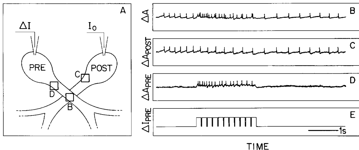
FIGURE 5 Optical recording of the activity of a pair of synaptically interacting LUQ neurons. These cells were coupled by an inhibitory synapse similar to that shown in Fig. 3. (A) Schematic diagram of the co-cultured neurons. The boxes correspond to the field observed by selected detectors in the photodiode array. A 2.0-s burst of action potentials were induced in the presynaptic cell by injecting intracellular current pulses, \Delta I(t) (2 nA in amplitude, 150 ms in duration at 180-ms intervals). The basal activity of the postsynaptic cell was set by an intracellular bias current I_0 . (B) Optical recording measured by an array element encompasses the neurites of both cells. The simultaneous activity of both neurons is seen. Note the decrease in firing rate of the postsynaptic neuron after stimulation of the presynaptic neuron. (C) Optical recording of the activity monitored in the initial segment of the postsynaptic neuron. (D) Optical recording of the activity monitored in the initial segment of the presynaptic neuron. (E) Time dependence of the current-pulse injected into the presynaptic cell.
