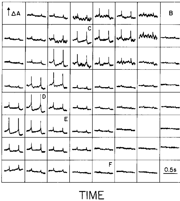
FIGURE 1 Optical recording of consecutive action potentials in an LUQ neuron, 3 d in vitro. The cell was bathed in normal ASW. (A) Photograph of the neuron using phase-contrast optics. The total field corresponds to an area measured by 64 detectors of the photodiode array. Each small square corresponds to the field observed by one of the detectors. (B) Optical recording of the electrical activity monitored in each of the detectors. (C) The activity monitored by a detector over the cell soma. (D) The activity monitored over the initial segment. Action potentials recorded by this detector had the largest S/N. (E) The activity monitored in a typical neurite. (F) The activity monitored in the finest neurites. Action potentials could not be observed in a single trace with this detector.
