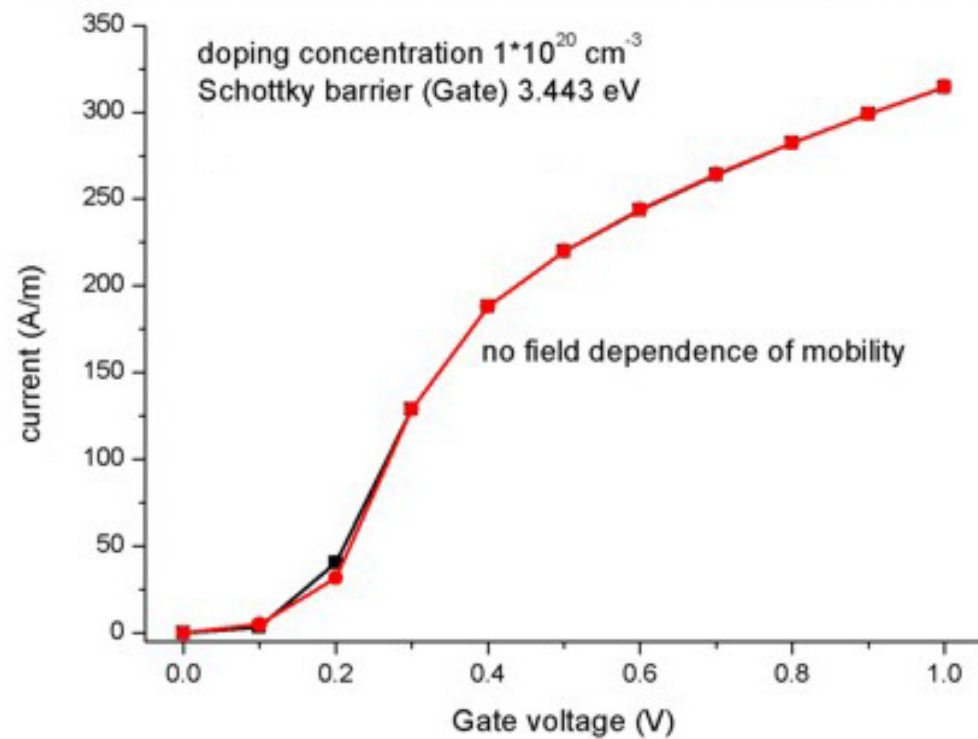
Current-voltage (I-V) characteristic of a 2 nm Si Double Gate MOSFET
