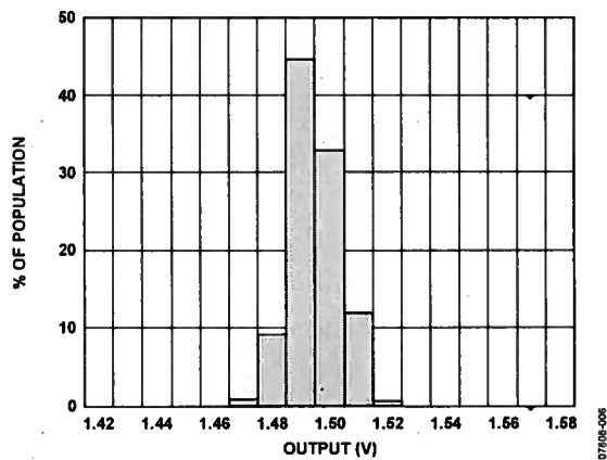
Figure 4. Y-Axis Zero g Bias at 25°C, V_S = 3 V
