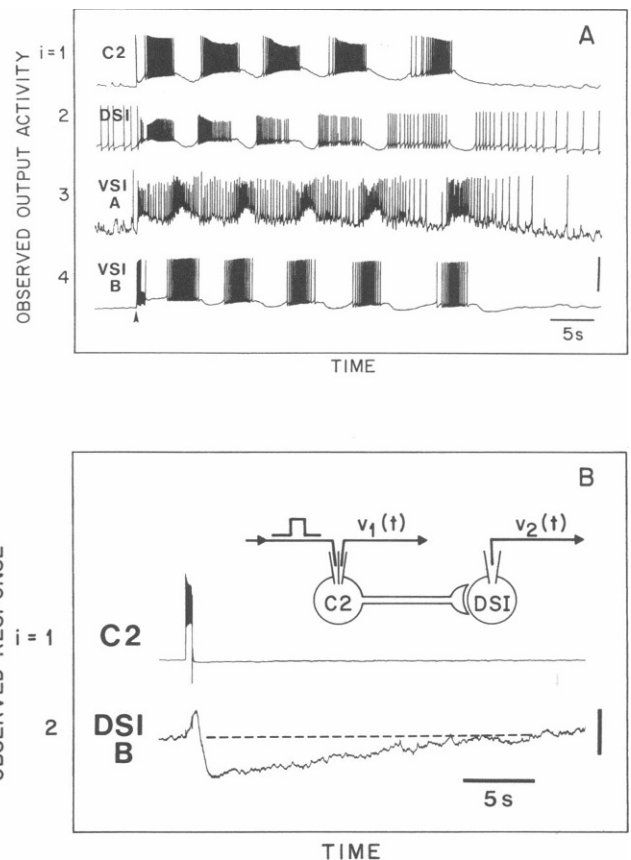
FIGURE 3 The observed behavior of the CPG controlling the escape swim response in Tritonia . (A) The output activity simultaneously measured from a C2 , DSI , VSI-A and VSI-B neuron in an isolated brain preparation from Tritonia . These neurons comprise the CPG that controls the escape swim sequence. Their output corresponds to V_1(t) , V_2(t) , V_3(t) , and V_4(t) , respectively, in the analysis presented in the text. Vertical bar: 50 mV for C2 , DSI and VSI-B and 25 mV for VSI-A . Adapted from Getting (25) with permission. (B) An example of the synaptic interaction between two neurons in the CPG in Tritonia . Shown is the presynaptic activity measured in the C2 neuron, v_1(t) , and the postsynaptic response measured in a DSI neuron, v_2(t) , as the result of a short pulse of current injected into C2 . The measurement was performed under conditions which insured that only monosynaptic connections contributed to the observation. The area under the initial, positive going response corresponds roughly to T_{21}^S , that under the slowly decaying response corresponds to T_{21}^L . The time dependence of the slow decay corresponds to the time dependence of w(t) . Vertical bar: 40 mV for C2 and 2 mV for DSI . Adapted from Getting (23) with permission.
